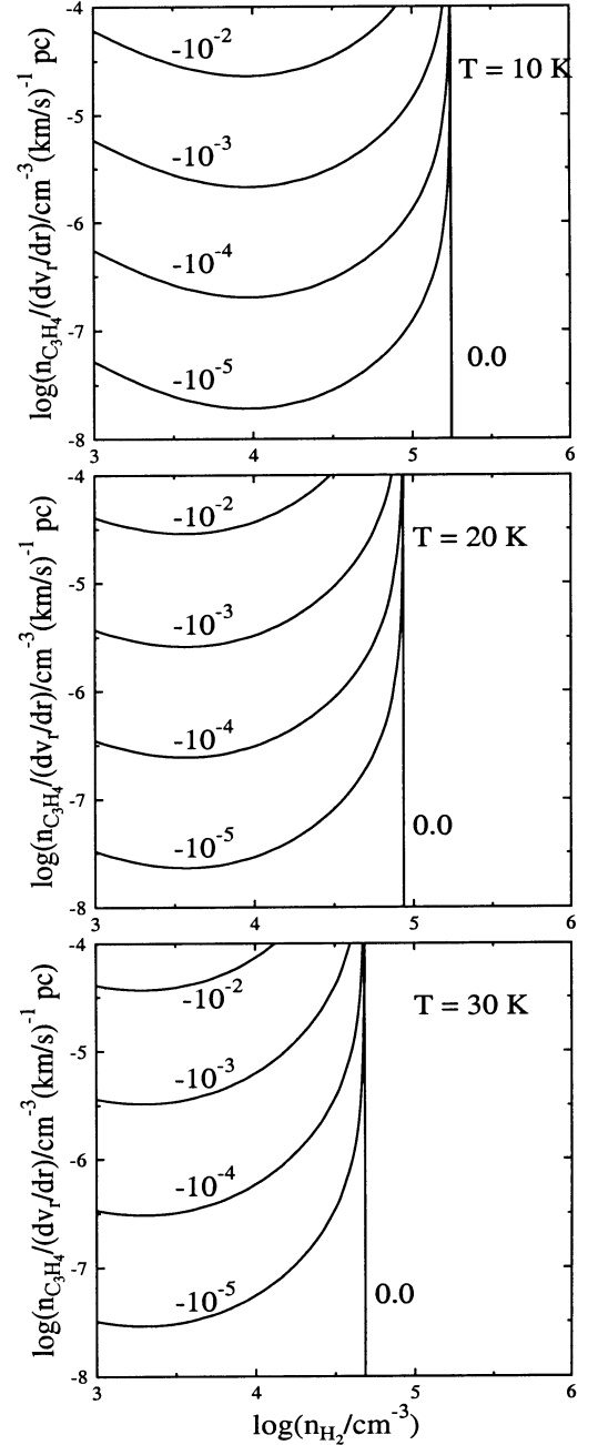
Fig. 2. The iso-lines for intensity against the cosmic 2.7 K background, in the unit of Planck's function at the kinetic temperature of T (K), i.e., (I_\nu - I_{\nu,\text{bg}})/B_\nu(T) , for the 2_{20}-2_{21} transition at 3.67218 GHz of para-C 3 H 4 . Only negative values for the kinetic temperatures T = 10, 20 , and 30 K are plotted. For large molecular hydrogen densities (where the iso-lines are not plotted), the value becomes positive.
