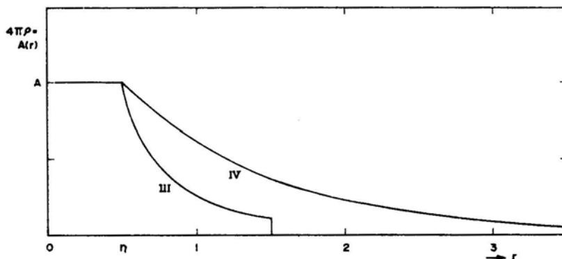
Figure 2. Behaviour of the reduced density 4\pi\rho/A . The curve labelled III corresponds to the definition of Section 3. One has here r_1 = 0.5 and r_2 = 1.5 . The curve labelled IV corresponds to the definitions of Section 4. One has there r_1 = 0.5 , B = 0 , C = 1 .
