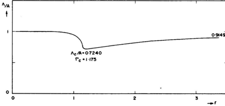
Figure 3. Typical Behaviour of \Lambda(r) . The curve of the figure corresponds to the variation of density described on curve IV, Fig. 2.
