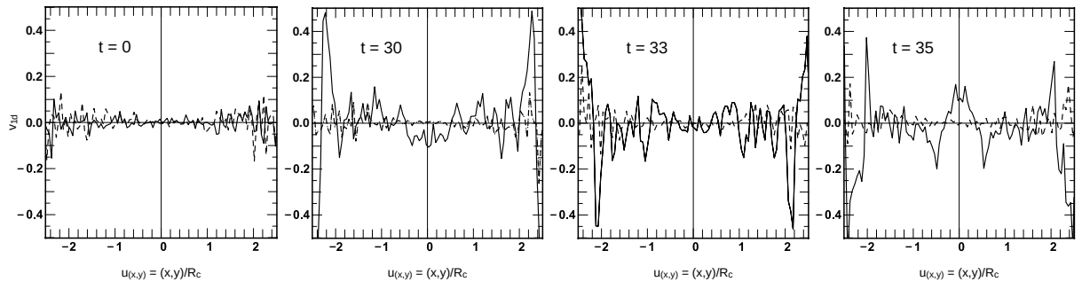
Figure 11. Time-sequence showing the line-of-sight mean velocity v_{1d} for the reference calculation with BH mass \tilde{m}_{bh} = 0.3 and amplitude u_0 = 0.33 . The velocity was measured when looking down the x -axis (solid line) and the y -axis (dashed line). The x -axis data show cyclical variations with a peak S/N inside u = 1 (or r = R_c ).
