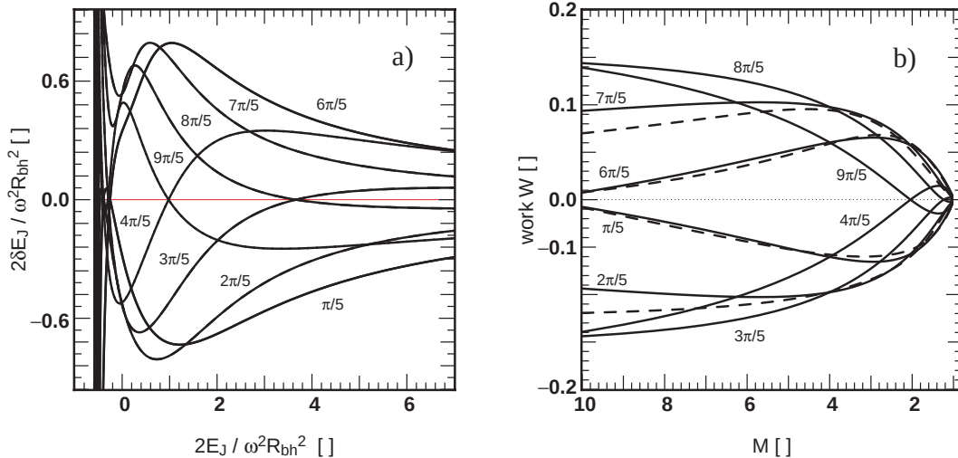
Figure 2. (a) Left-hand panel: energy increment \delta E_J for one revolution as a function of the initial orbital energy, E_J . The curves are labelled with eight values of the phase angle \phi_0 . The calculation was done in units where G = \omega = 1 with a BH mass M_{\text{bh}} = 0.07 . The influence radius R_{\text{bh}} \simeq 0.42 in those units. Both \delta E_J and E_J are given as ratios of the kinetic energy of an oscillator of amplitude R_{\text{bh}} . (b) Right-hand panel: net work W as a function of M defined in equation (8). The solid lines are the relation (13) for the same eight values of \phi_0 as in panel (a). The dash was computed using both first and second orders of a Taylor expansion, cf. equation (B6).
