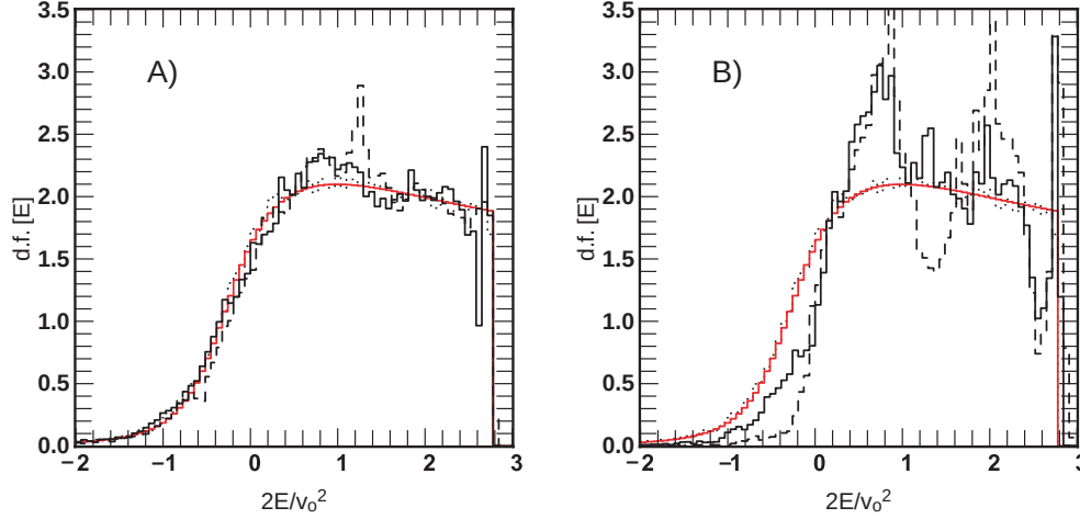
Figure 13. This graphs the energy distribution for four values of the BH’s amplitude of motion u_0 = R_0/R_c . The dimensionless mass parameter \tilde{m}_{bh} = 0.3 in all the cases. In panel (a) we plot two solutions with u_0 = 0.07 (solid line) and 0.15 (dashed line); in panel (b) we set u_0 = 0.21 (solid line) and 0.30 (dashed line). The smooth histogram is the analytic solution (28). The dots show a discrete realization with 69 977 orbits and u_0 = 0 (axially symmetric potential). The energy 2 E_J/v_0^2 \simeq -0.54 corresponds to \alpha = u_0/u = 1 .
