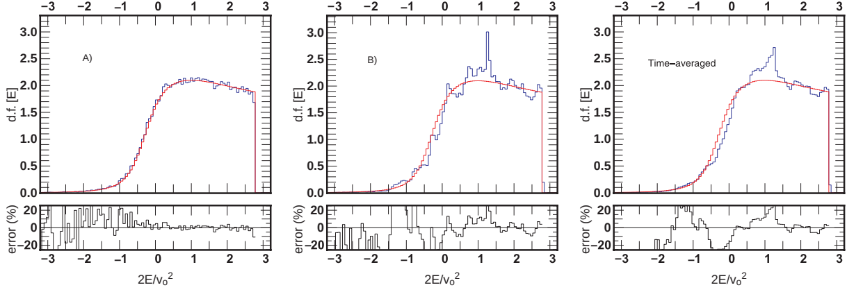
Figure 7. Energy distribution for two configurations: (a) static BH at the centre of coordinates; (b) BH on a radial orbit of amplitude u_o = 0.33 , after 40 time-units of evolution. In both cases, the mass parameter \tilde{m}_{bh} = 0.3 . The energy distribution function averaged over five output times is shown in the right-hand side for comparison. The smooth histogram on all three panels was constructed using equation (32).
