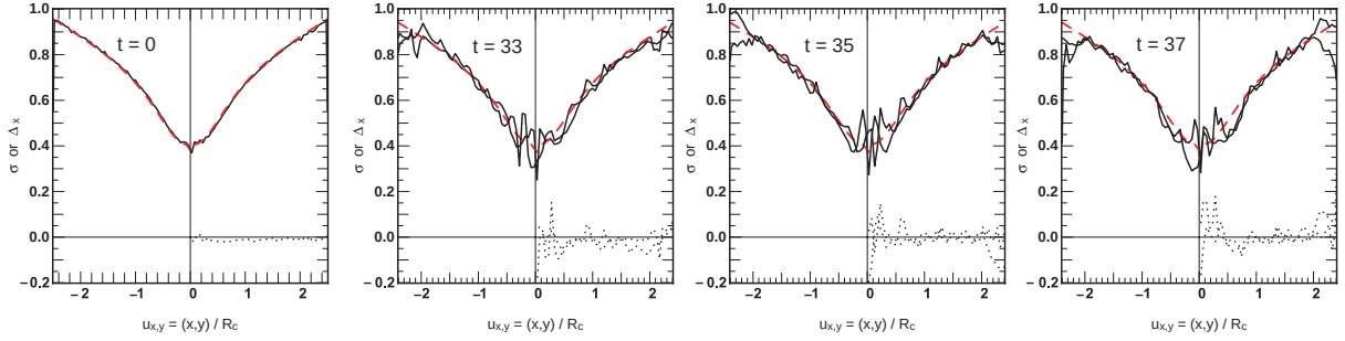
Figure 10. Time-sequence showing the line-of-sight rms velocity dispersion, \sigma_{1d} , for case C3 with \tilde{m}_{bh} = 0.3 \simeq u_0 . A total of 100 bins were used for two viewing angles, down the x -axis and y -axis, in each case. At t = 0 (panel to the extreme left-hand side), the analytic expectation with a BH at the centre of coordinates is well recovered from 69 773 circular orbits. The dashed line shows the theoretical expectations which drop to zero at the origin (all motion is orthogonal to the line of sight). The solid line gives the dispersion recovered from summing over all orbits. The thin dotted lines are the differences about the coordinate centre \Delta = \sigma(u) - \sigma(-u) for each line of sight.
